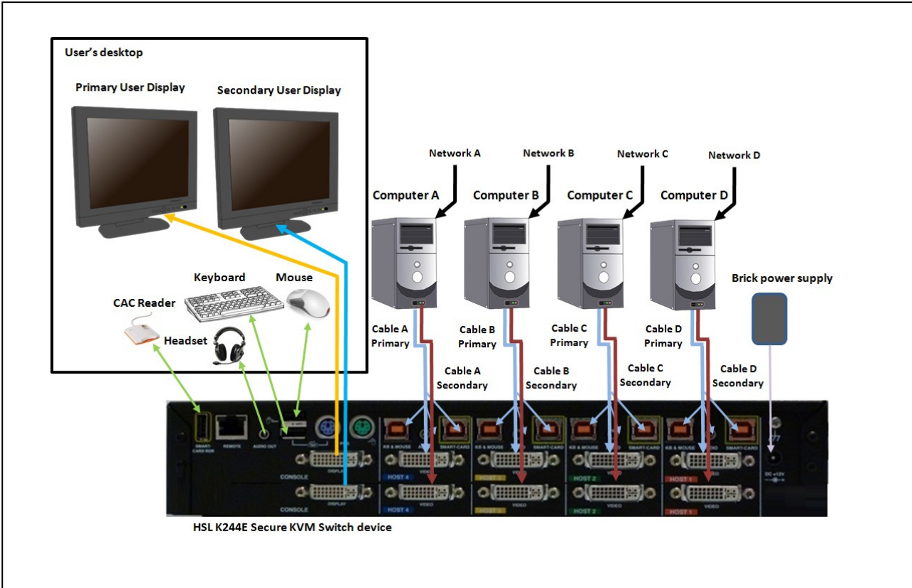
K244E typical system diagram
